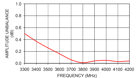
NCS4-442+ AMPLITUDE UNBALANCE
