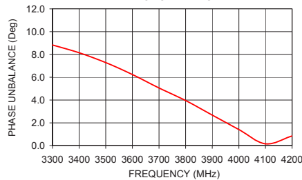
NCS4-442+ PHASE UNBALANCE
