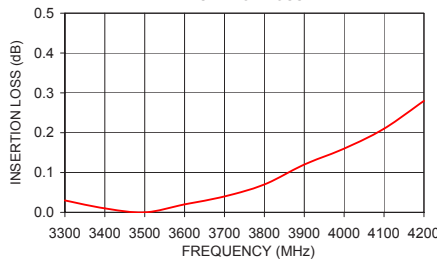
NCS4-442+ INSERTION LOSS*
