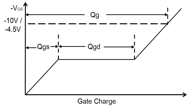
Figure 8. Gate Charge Waveform
