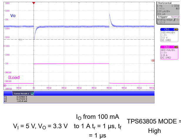
Figure 10-38. Load Transient, PWM Buck Operation
