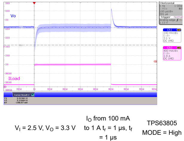
Figure 10-36. Load Transient, PWM Boost Operation
