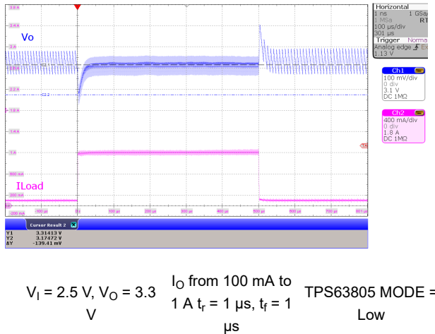
Figure 10-33. Load Transient, PFM/PWM Boost Operation
