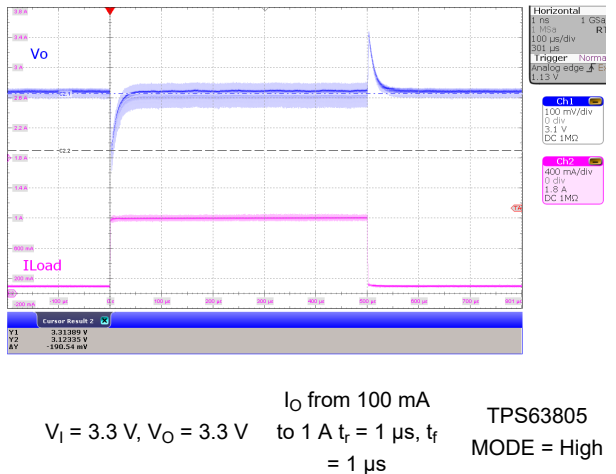
Figure 10-37. Load Transient, PWM Buck-Boost Operation
