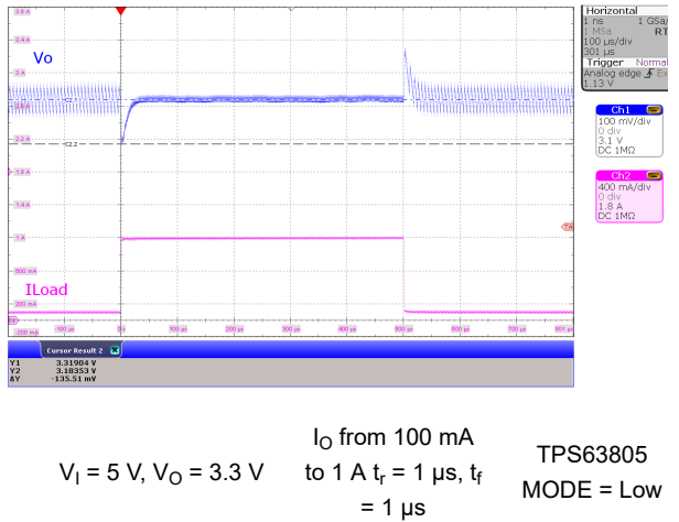
Figure 10-35. Load Transient, PFM/PWM Buck Operation
