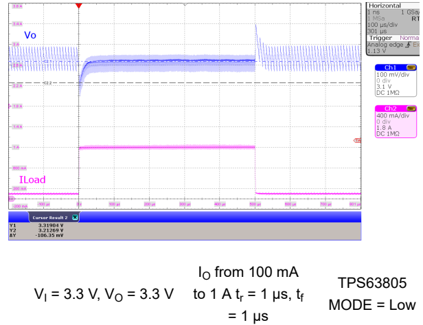
Figure 10-34. Load Transient, PFM/PWM Buck-Boost Operation
