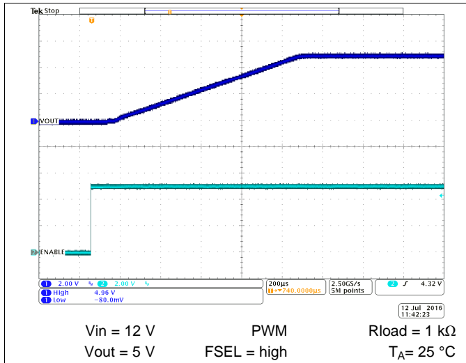
Figure 60. Start-Up Timing
