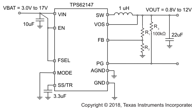
Figure 3. Measurement Setup with FSEL = high
