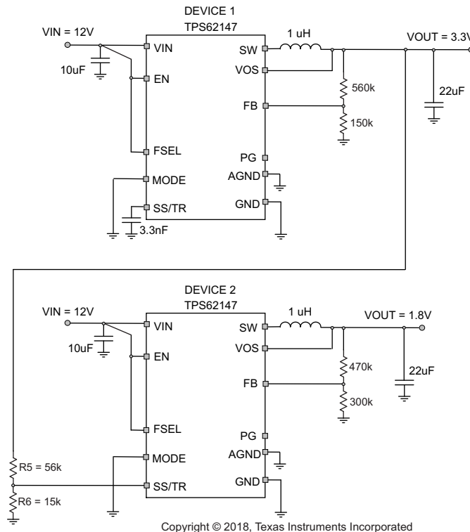
Figure 88. Tracking Example
