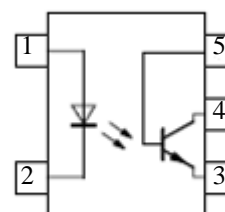
Pin Configuration
