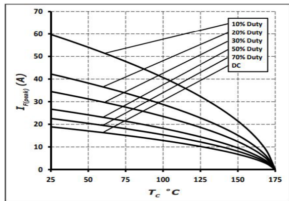
Figure 3 Current Derating
