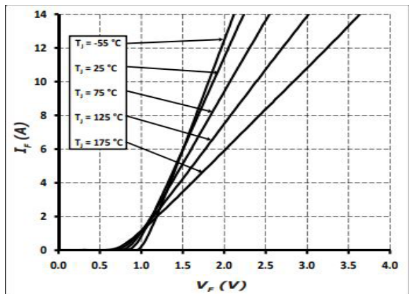
Figure 1 Forward Characteristics
