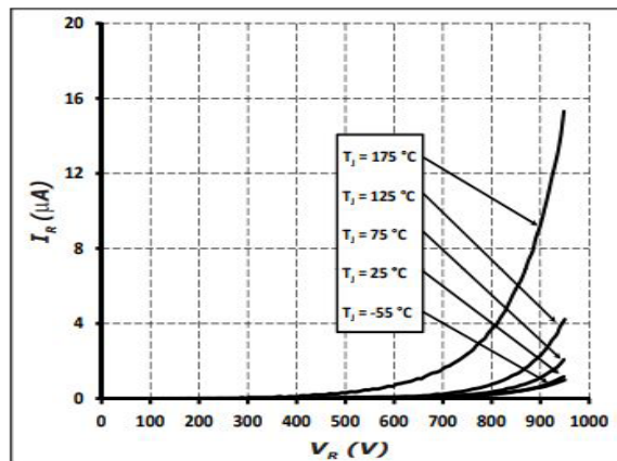
Figure 2 Reverse Characteristics
