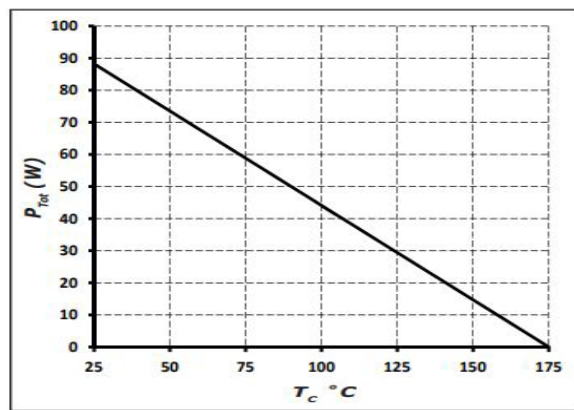
Figure 4 Power Derating
