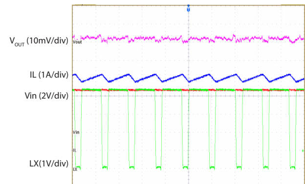
Vout Ripple ( V_{in}=5\text{V} , V_{OUT} = 3.3\text{V} ) @ Full Load
