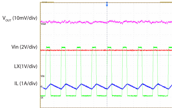
Vout Ripple ( V_{in}=5\text{V} , V_{OUT}=1.5\text{V} ) @0A Load
