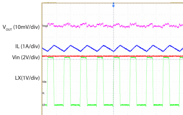
Vout Ripple ( V_{in}=5\text{V} , V_{OUT}=1.5\text{V} ) @ Full Load
