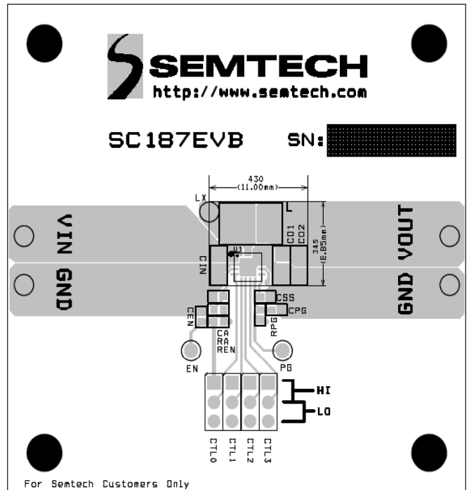
Figure 2 — Recommended PCB Layout (Top Layer)
