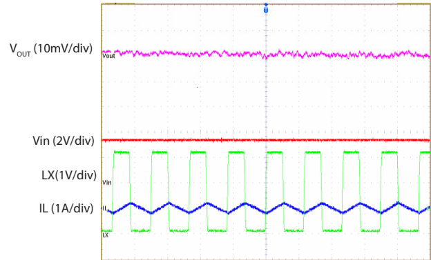
Vout Ripple ( V_{in}=3.3\text{V} , V_{OUT}=1.5\text{V} ) @ 0A Load
