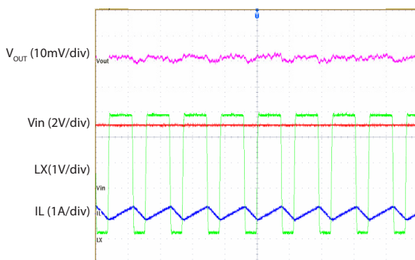
Vout Ripple ( V_{in}=5\text{V} , V_{OUT} = 3.3\text{V} ) @ No Load
