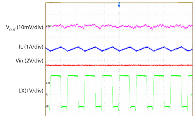
Vout Ripple ( V_{in}=3.3\text{V} , V_{OUT}=1.5\text{V} ) @ Full Load
