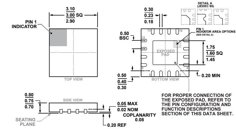
Figure 48. 16-Lead Lead Frame Chip Scale Package [LFCSP] 3 mm × 3 mm Body and 0.75 mm Package Height (CP-16-27) Dimensions shown in millimeters
