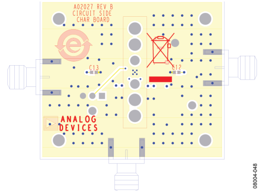
Figure 47. Layout of Evaluation Board, Circuit Side
